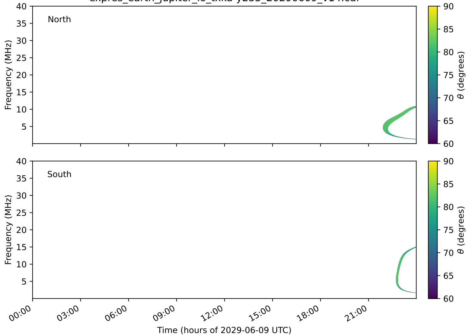
expres_earth_jupiter_io_txka-y235_20290609_v14.cdf
