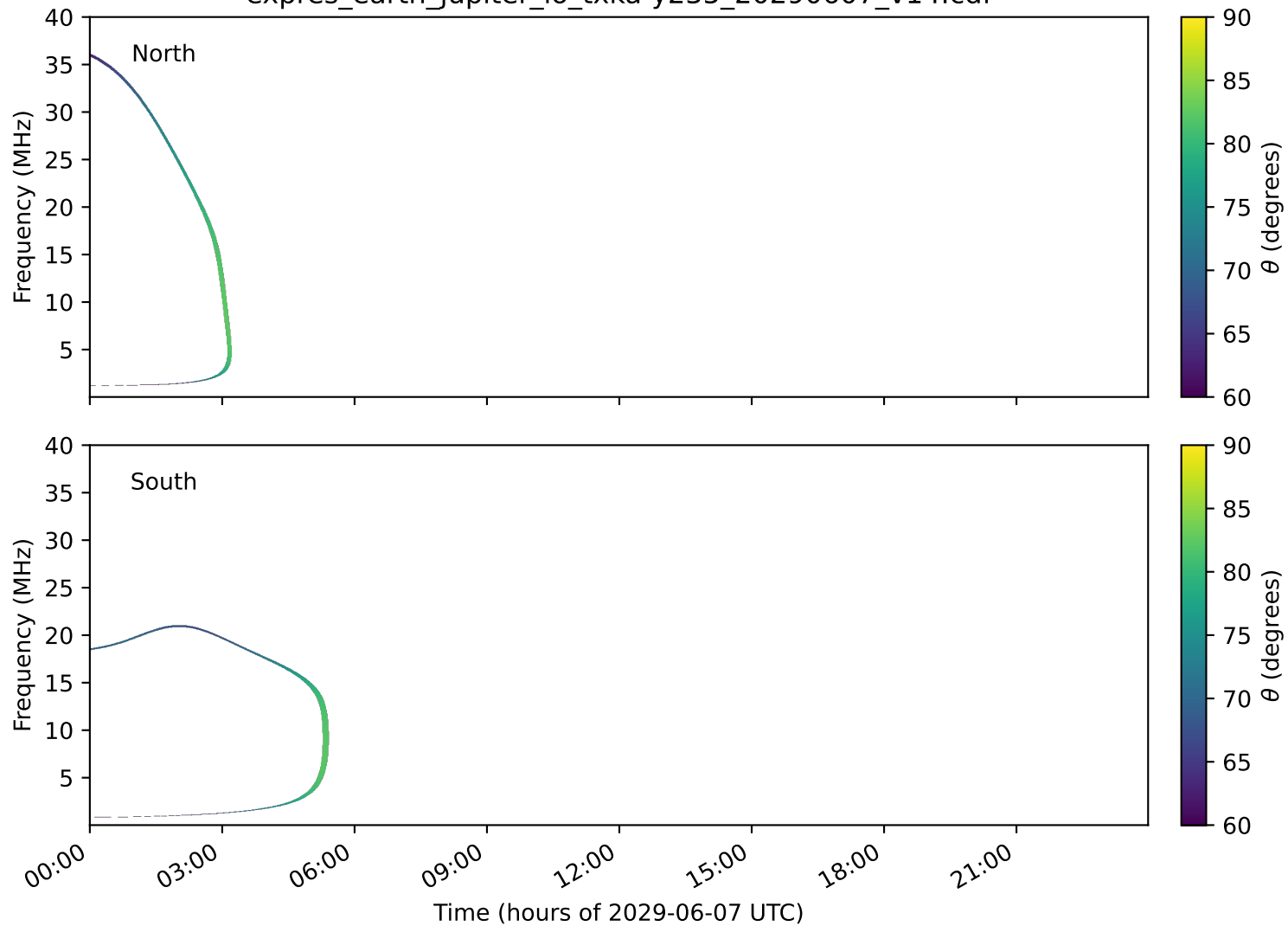
expres_earth_jupiter_io_txka-y235_20290607_v14.cdf
