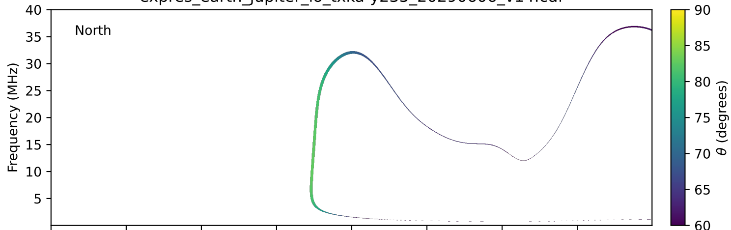
expres_earth_jupiter_io_txka-y235_20290606_v14.cdf
