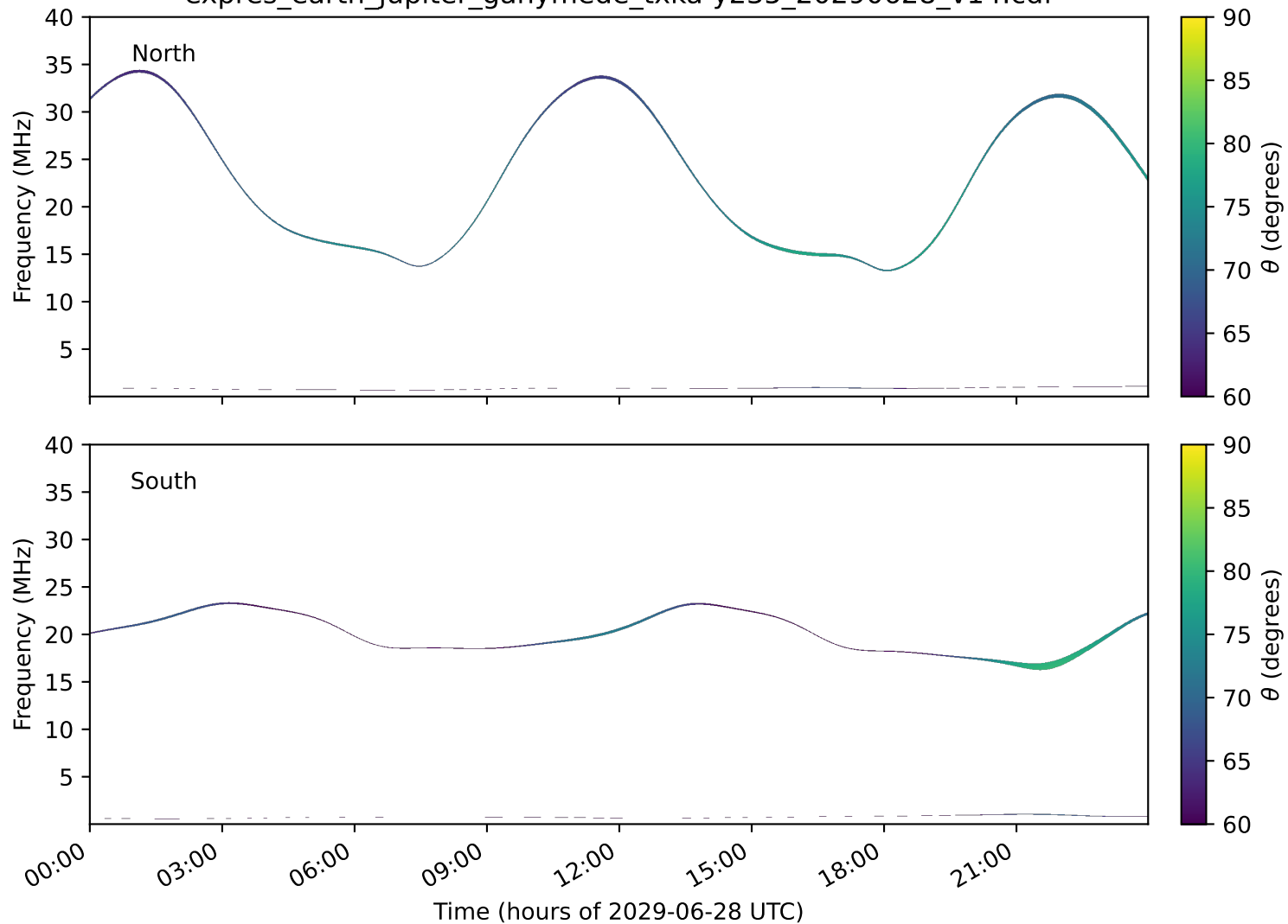
expres_earth_jupiter_ganymede_txka-y235_20290628_v14.cdf
