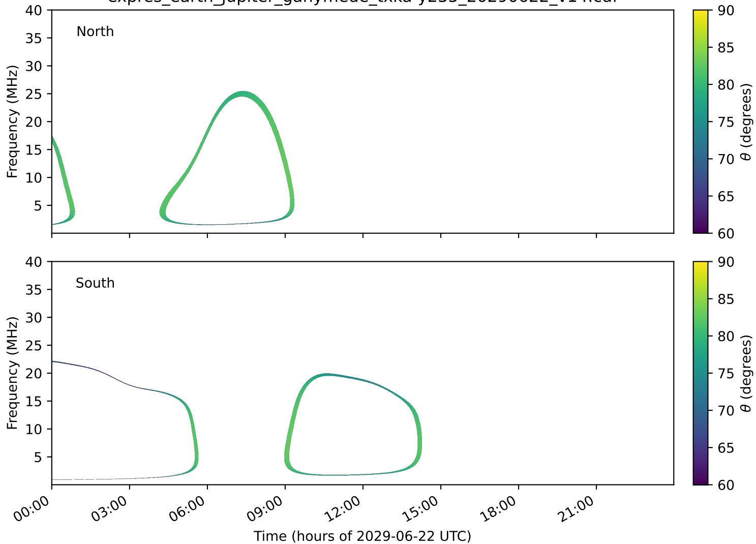
expres_earth_jupiter_ganymede_txka-y235_20290622_v14.cdf
