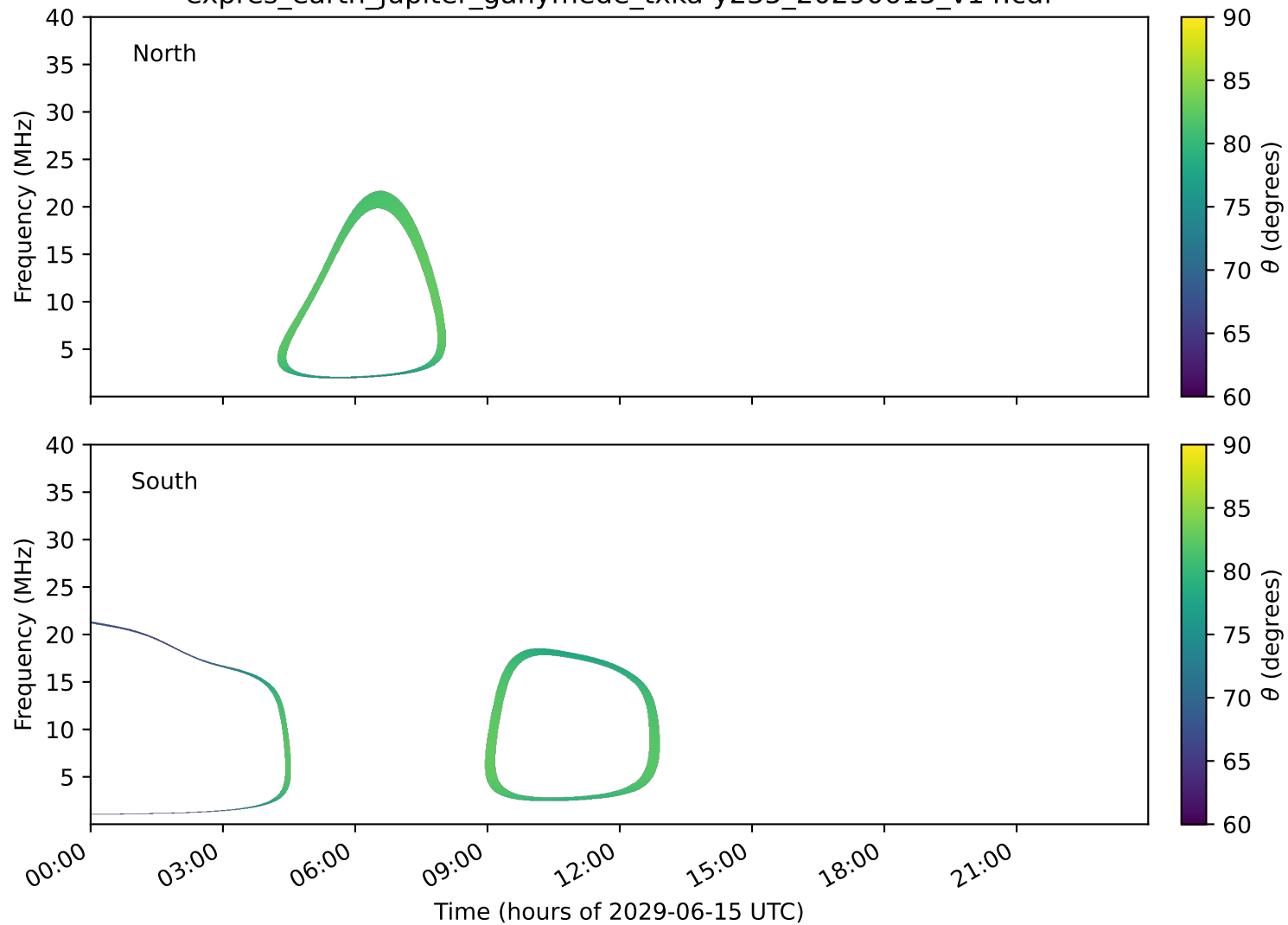
expres_earth_jupiter_ganymede_txka-y235_20290615_v14.cdf
