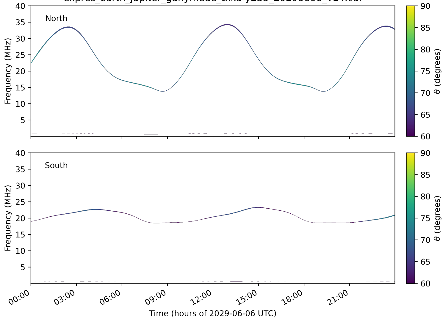
expres_earth_jupiter_ganymede_txka-y235_20290606_v14.cdf
