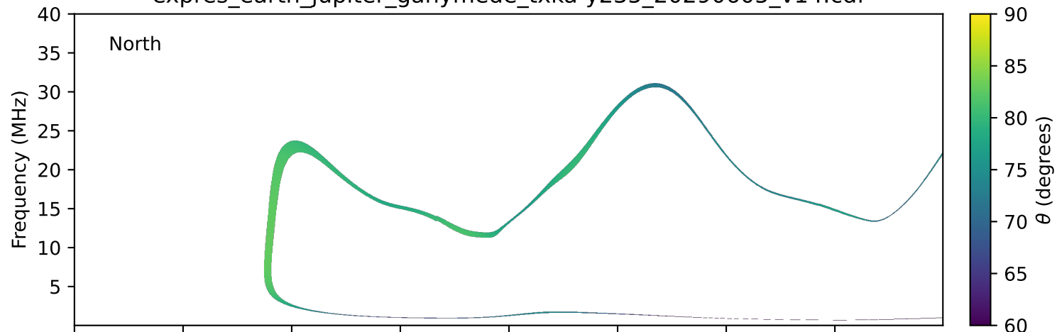
expres_earth_jupiter_ganymede_txka-y235_20290605_v14.cdf
