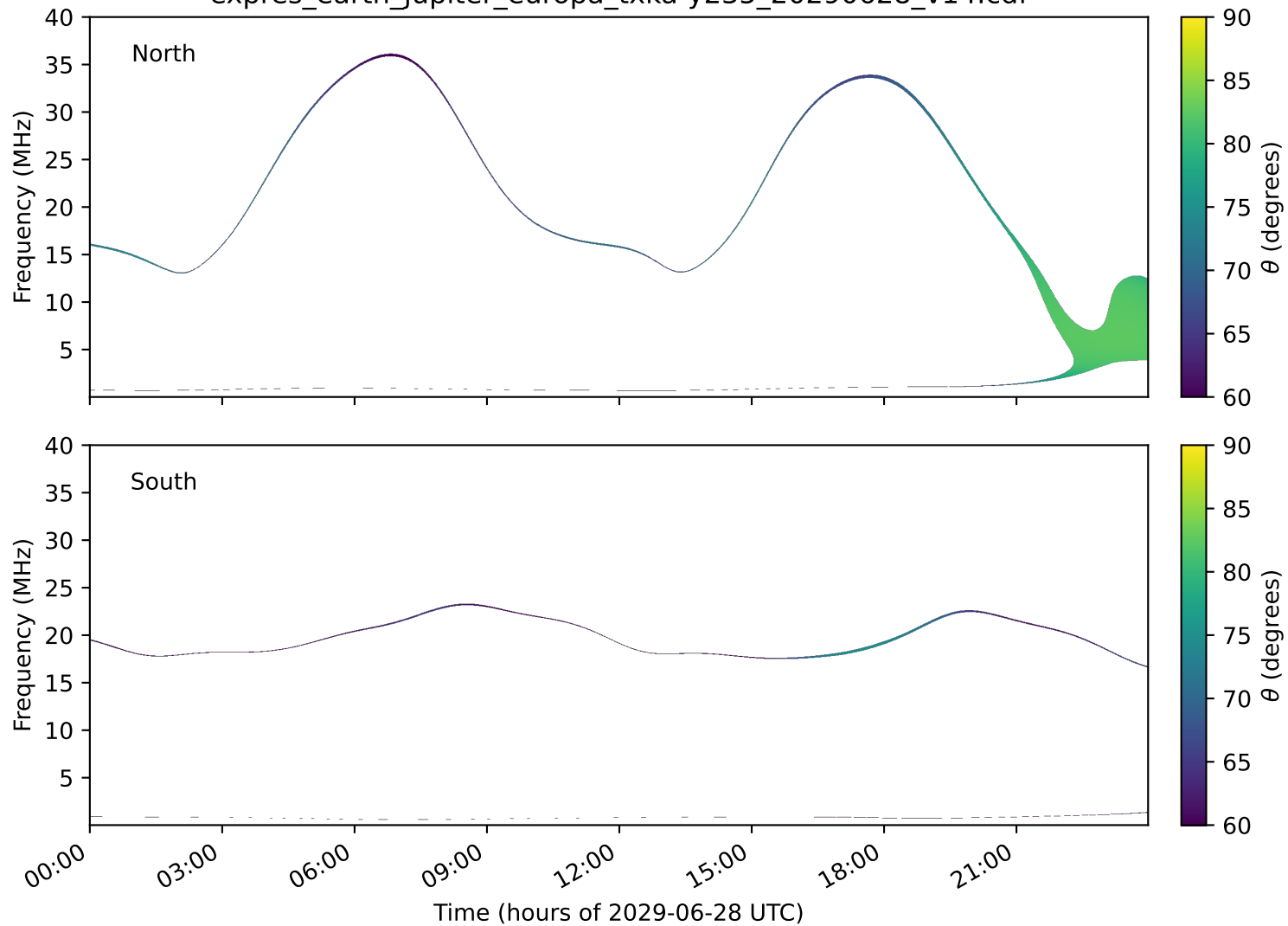
expres_earth_jupiter_europa_txka-y235_20290628_v14.cdf
