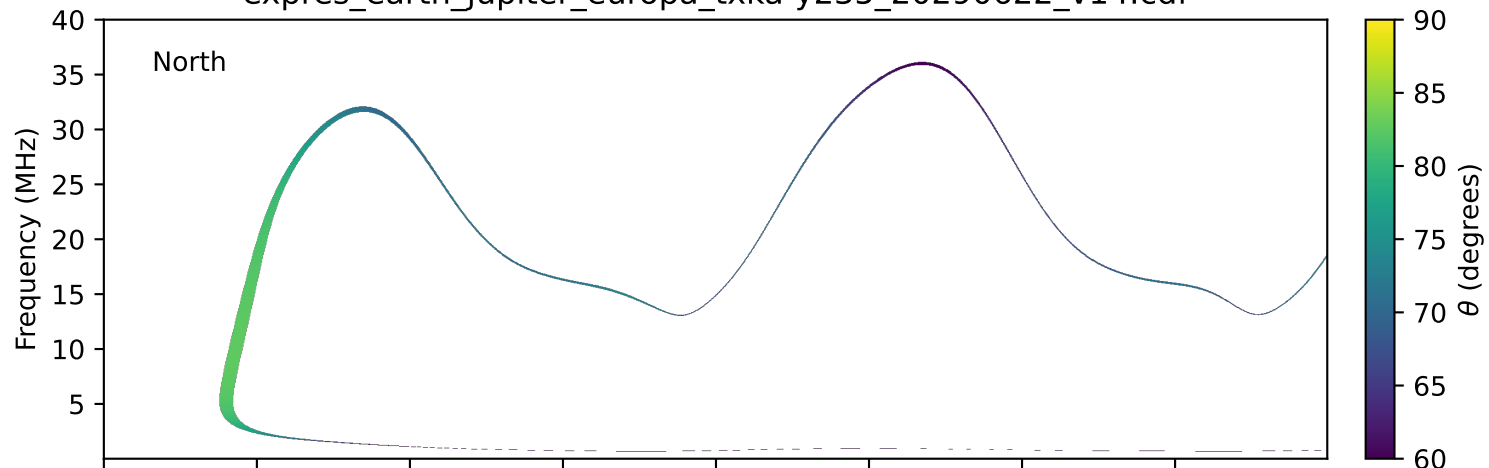
expres_earth_jupiter_europa_txka-y235_20290622_v14.cdf
