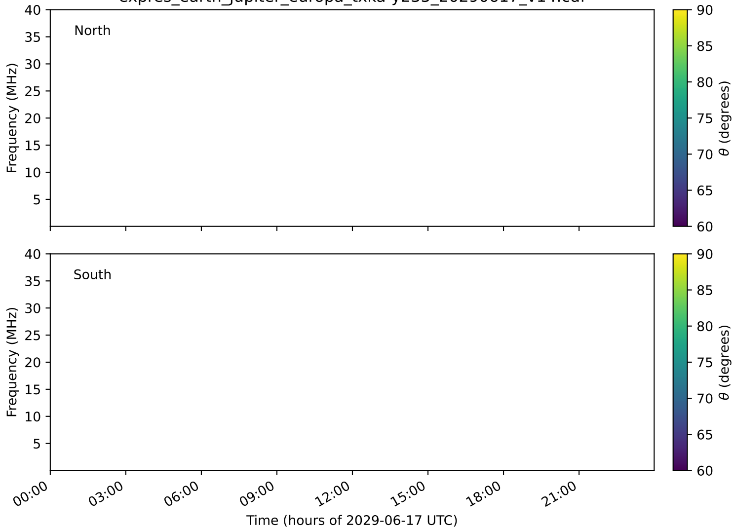
expres_earth_jupiter_europa_txka-y235_20290617_v14.cdf
