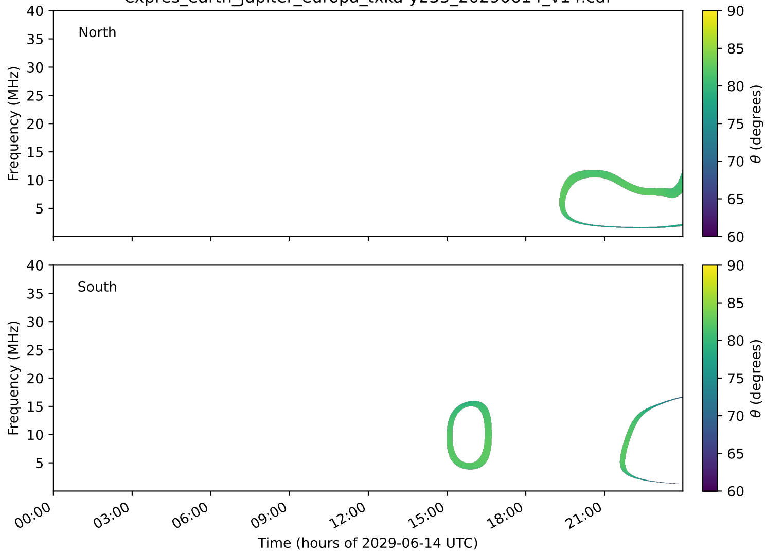
expres_earth_jupiter_europa_txka-y235_20290614_v14.cdf
