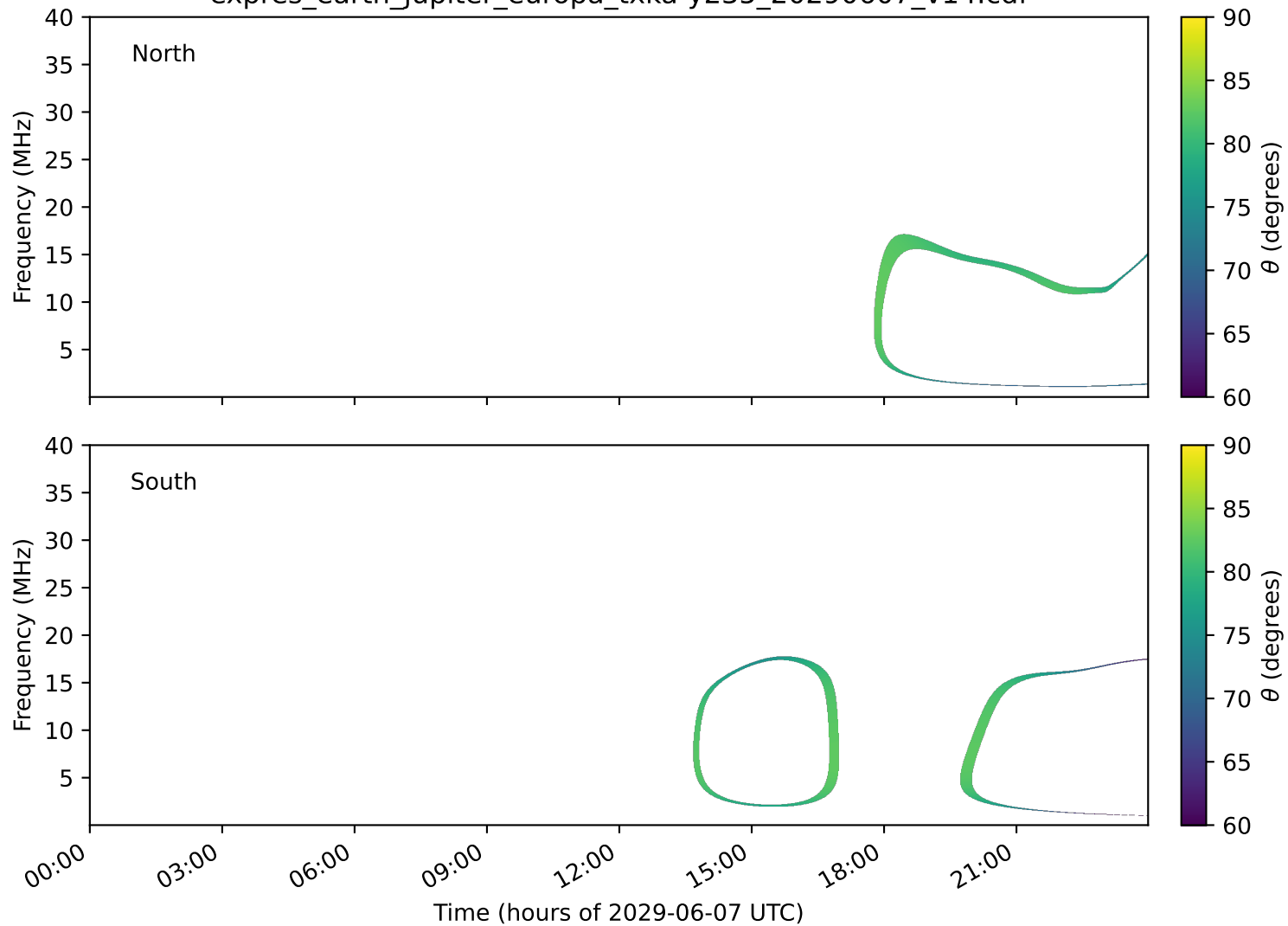
expres_earth_jupiter_europa_txka-y235_20290607_v14.cdf
