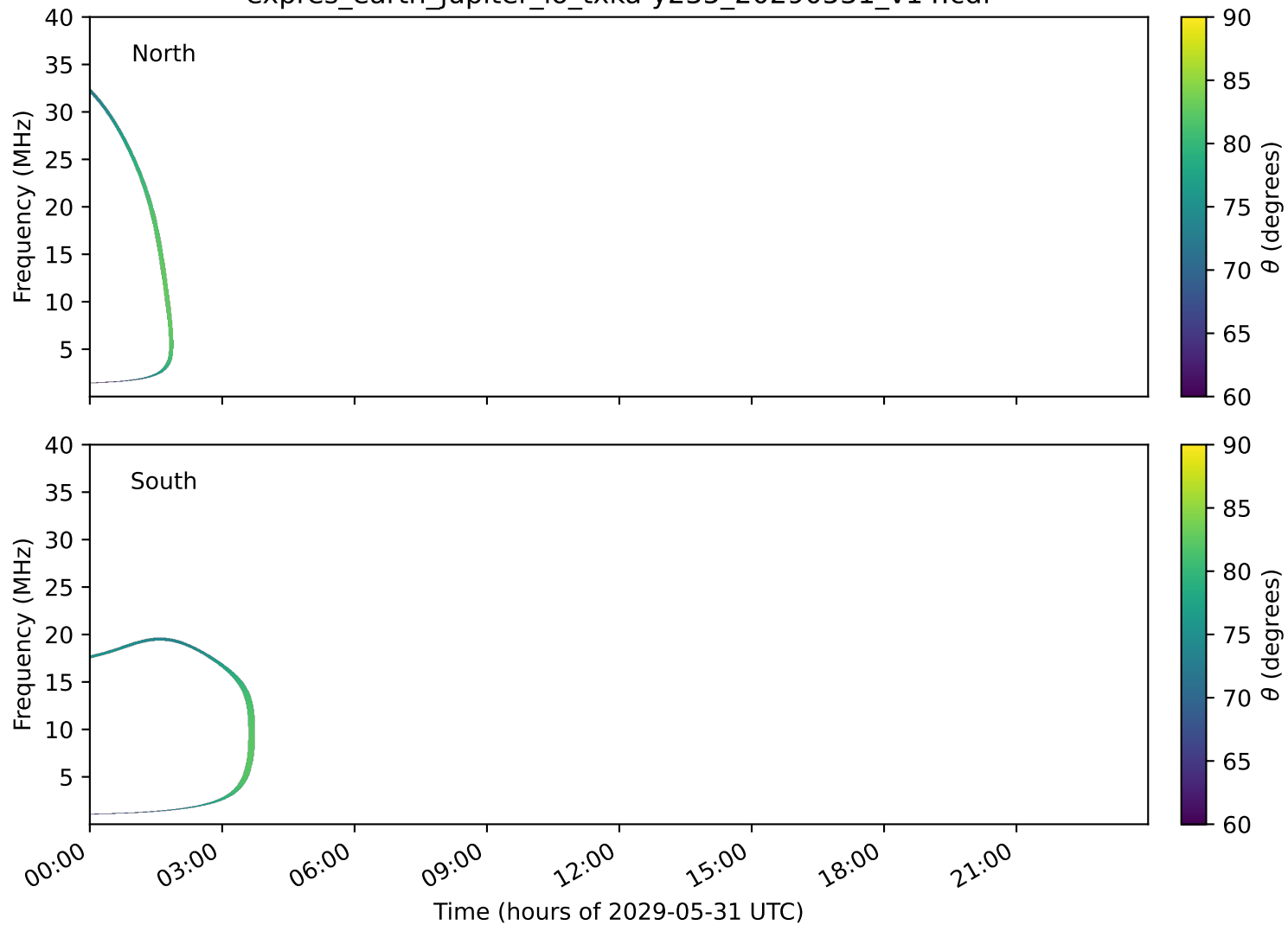
expres_earth_jupiter_io_txka-y235_20290531_v14.cdf
