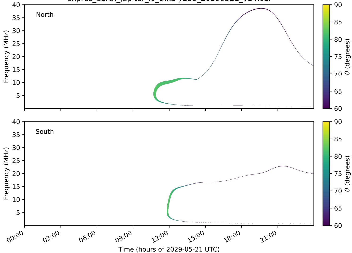
expres_earth_jupiter_io_txka-y235_20290521_v14.cdf
