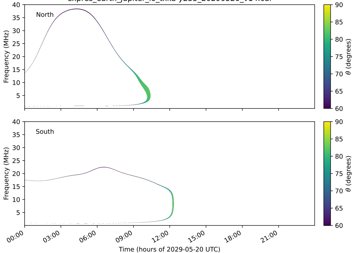
expres_earth_jupiter_io_txka-y235_20290520_v14.cdf
