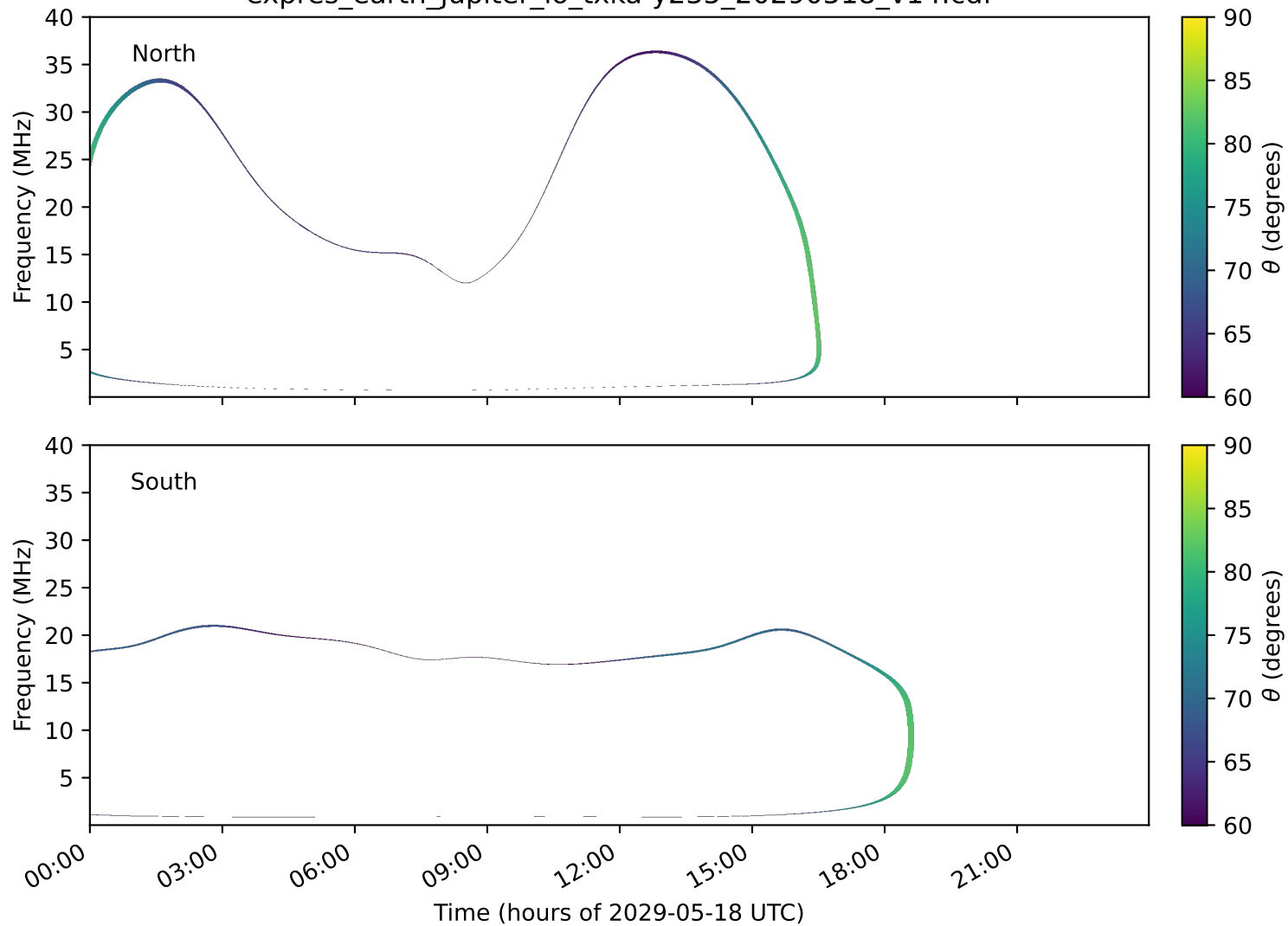
expres_earth_jupiter_io_txka-y235_20290518_v14.cdf
