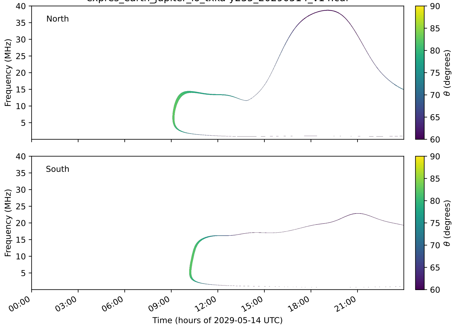
expres_earth_jupiter_io_txka-y235_20290514_v14.cdf
