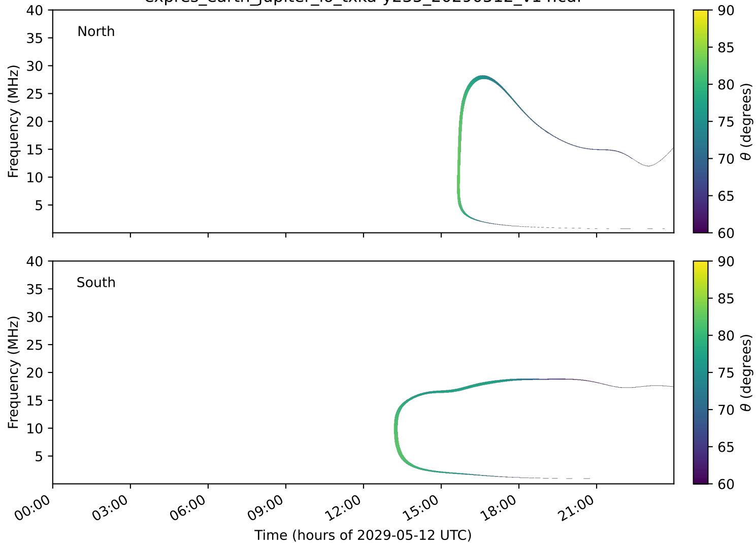
expres_earth_jupiter_io_txka-y235_20290512_v14.cdf
