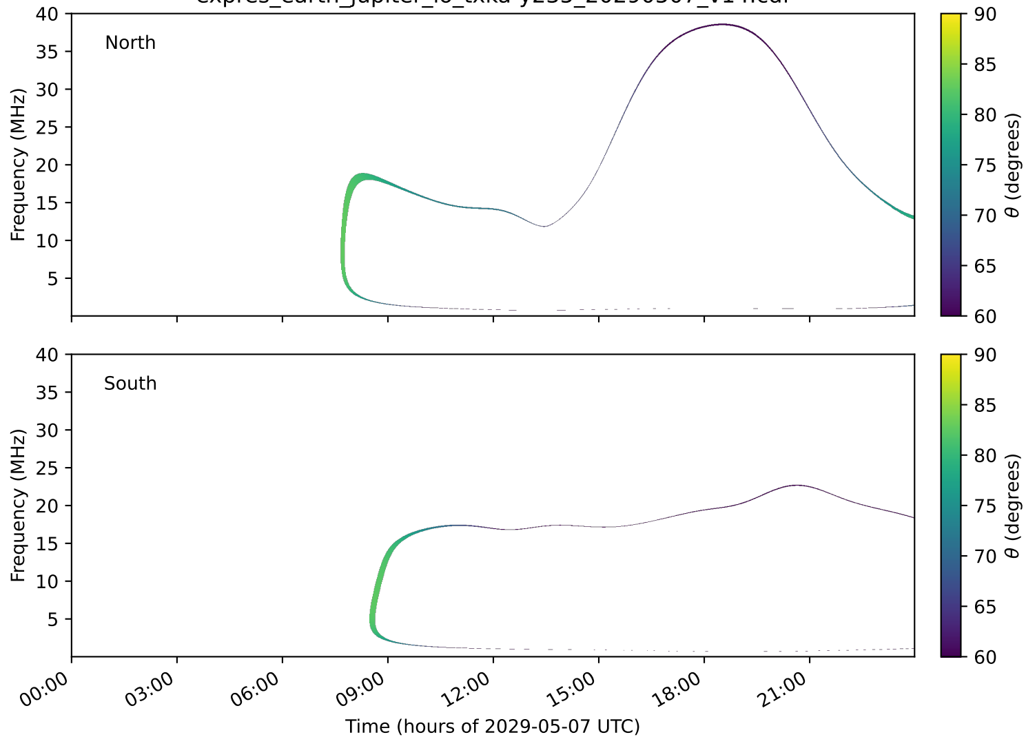
expres_earth_jupiter_io_txka-y235_20290507_v14.cdf
