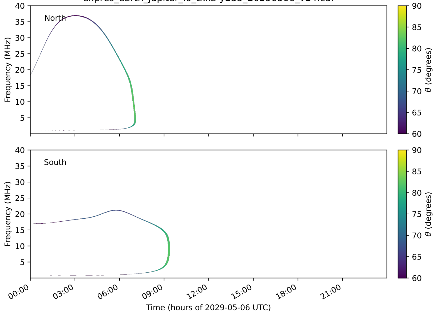
expres_earth_jupiter_io_txka-y235_20290506_v14.cdf
