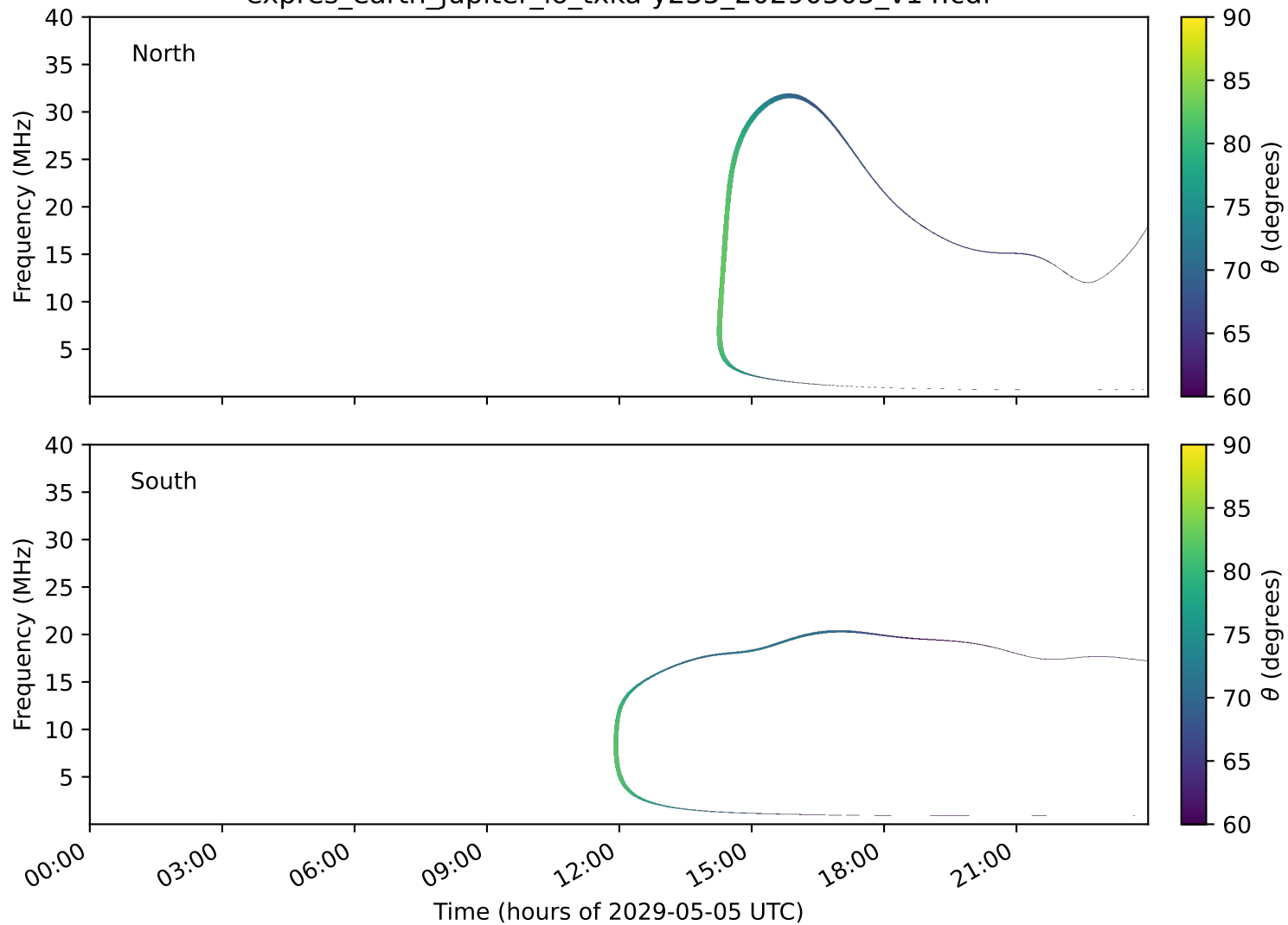
expres_earth_jupiter_io_txka-y235_20290505_v14.cdf
