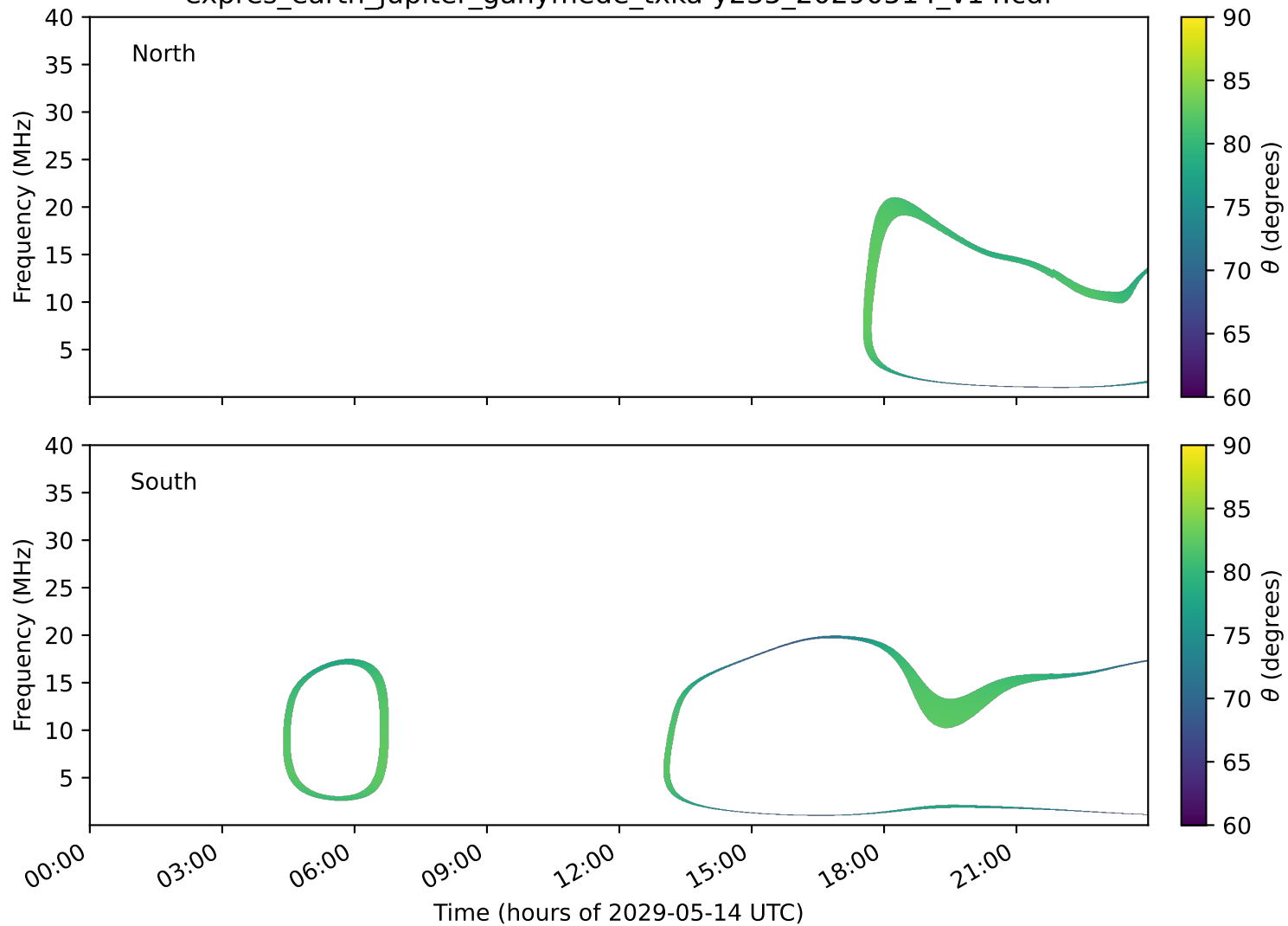
expres_earth_jupiter_ganymede_txka-y235_20290514_v14.cdf
