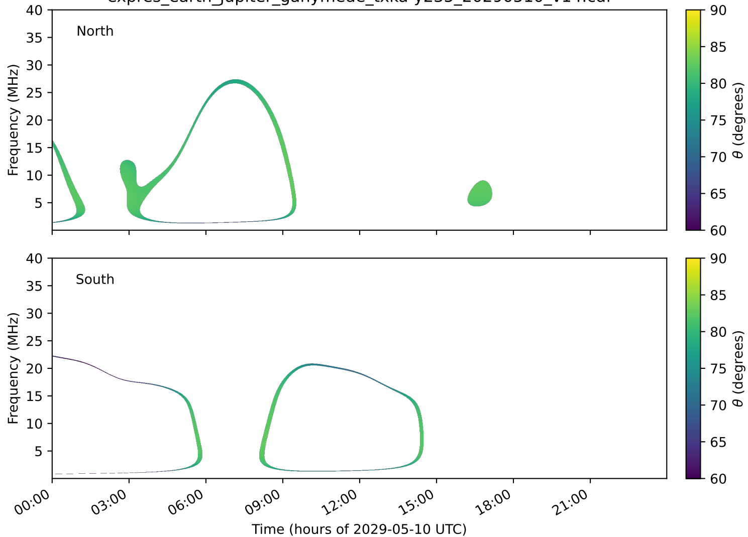
expres_earth_jupiter_ganymede_txka-y235_20290510_v14.cdf
