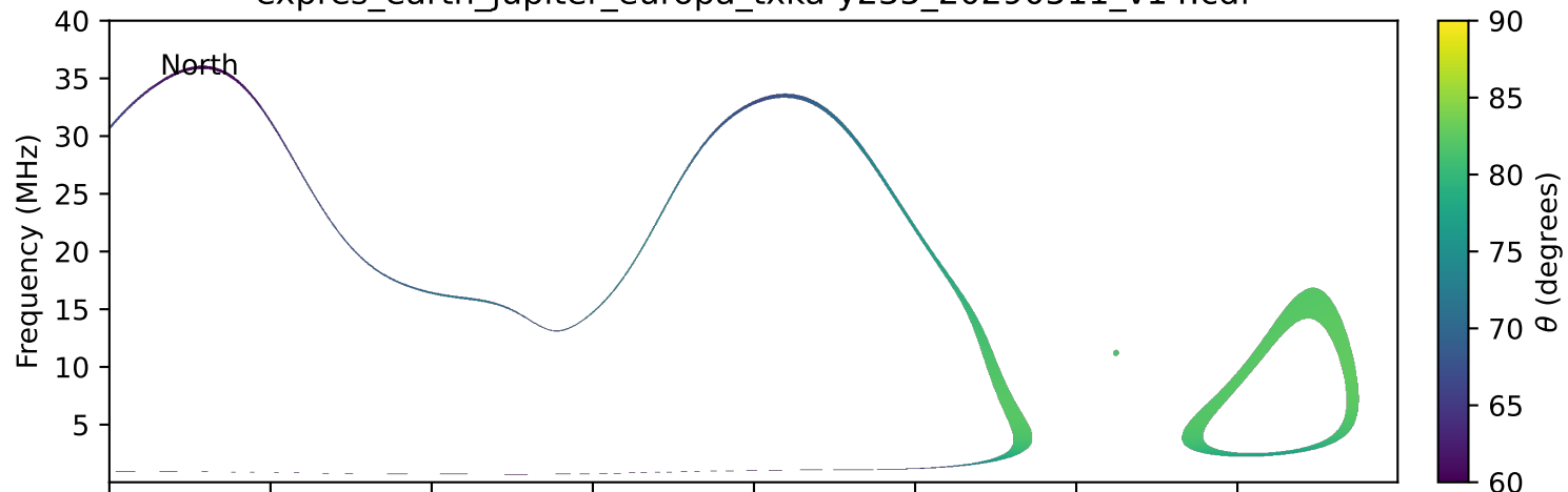
expres_earth_jupiter_europa_txka-y235_20290511_v14.cdf
