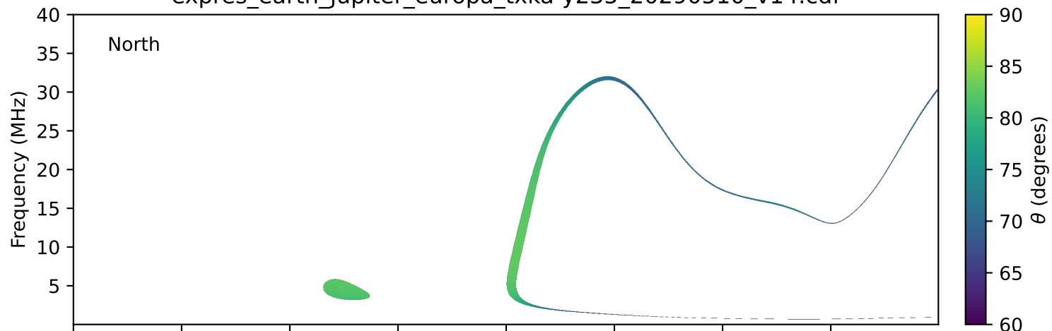
expres_earth_jupiter_europa_txka-y235_20290510_v14.cdf
