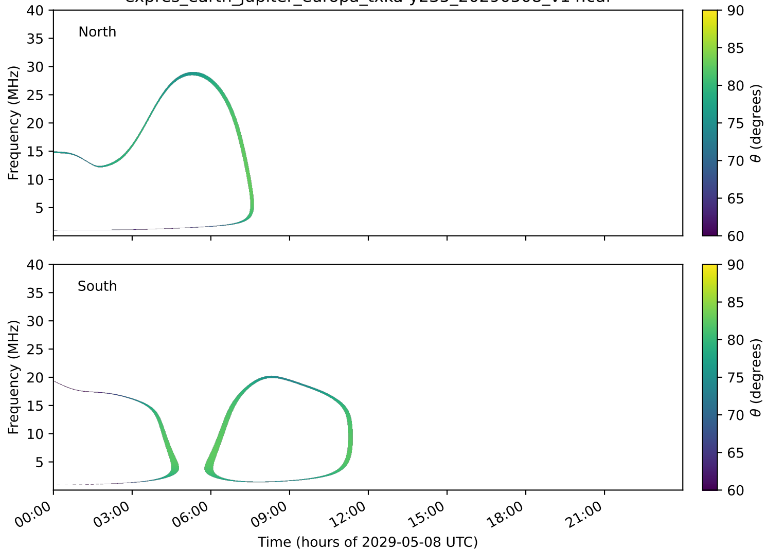
expres_earth_jupiter_europa_txka-y235_20290508_v14.cdf
