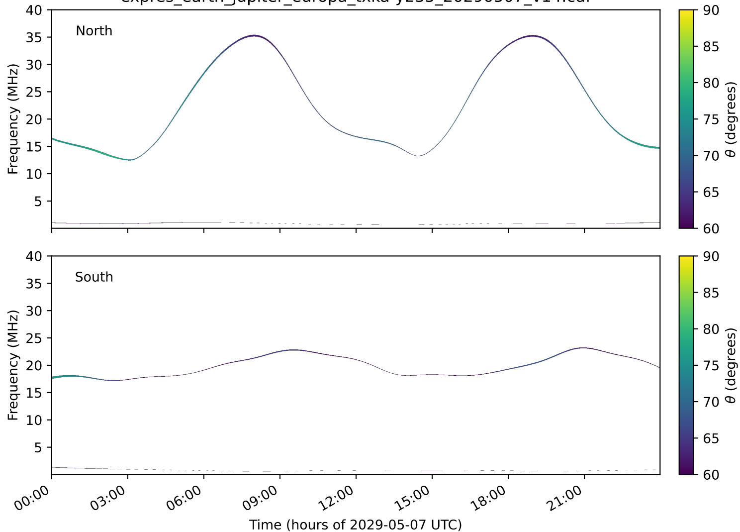
expres_earth_jupiter_europa_txka-y235_20290507_v14.cdf
