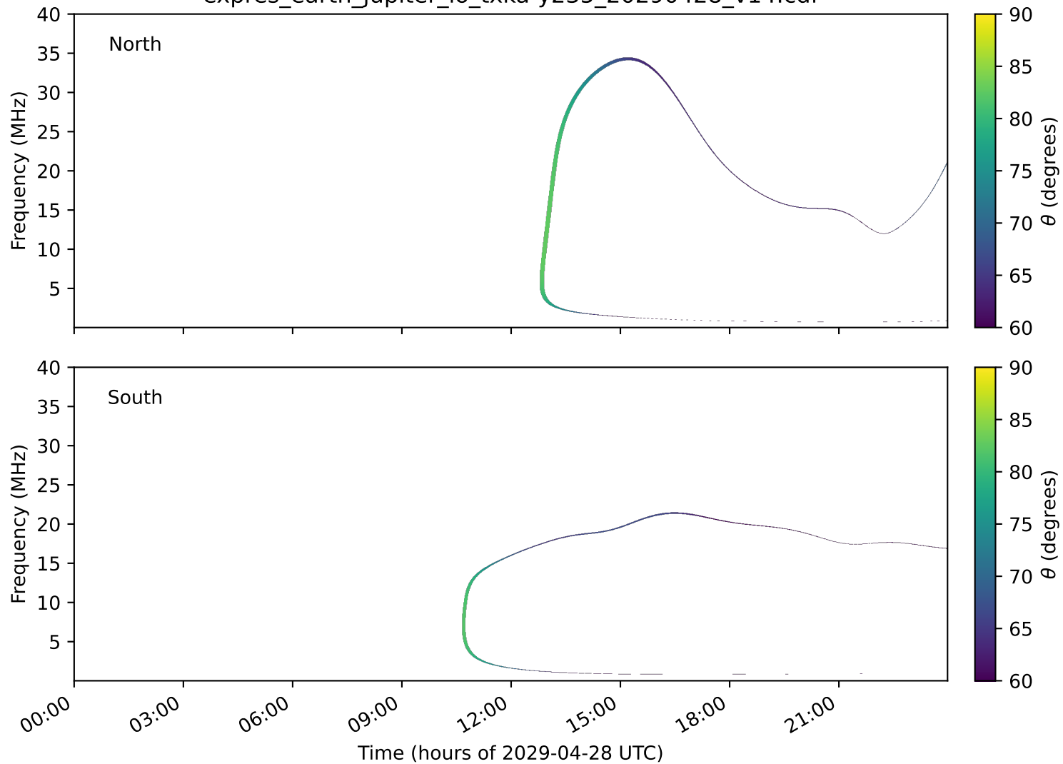
expres_earth_jupiter_io_txka-y235_20290428_v14.cdf
