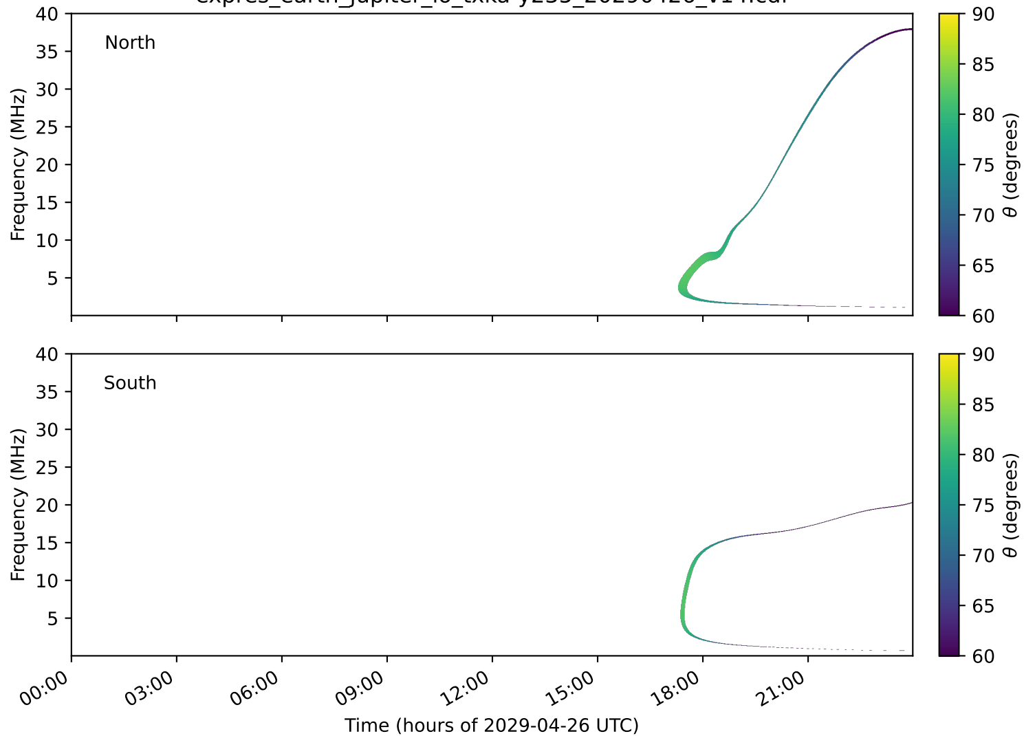
expres_earth_jupiter_io_txka-y235_20290426_v14.cdf
