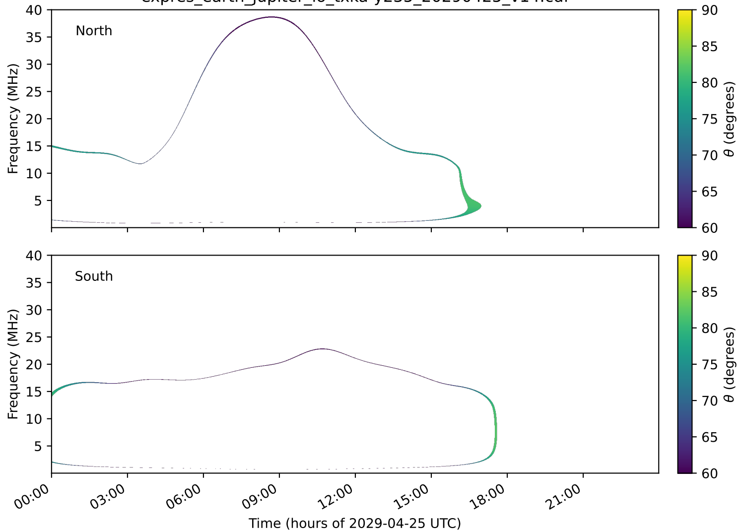
expres_earth_jupiter_io_txka-y235_20290425_v14.cdf
