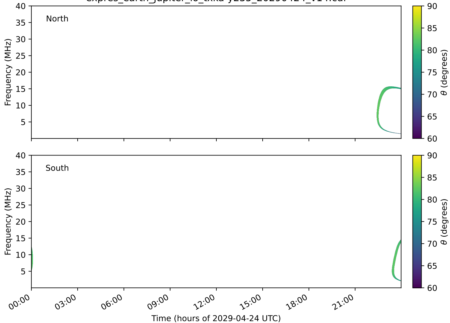
expres_earth_jupiter_io_txka-y235_20290424_v14.cdf
