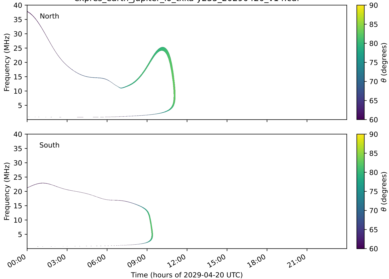
expres_earth_jupiter_io_txka-y235_20290420_v14.cdf
