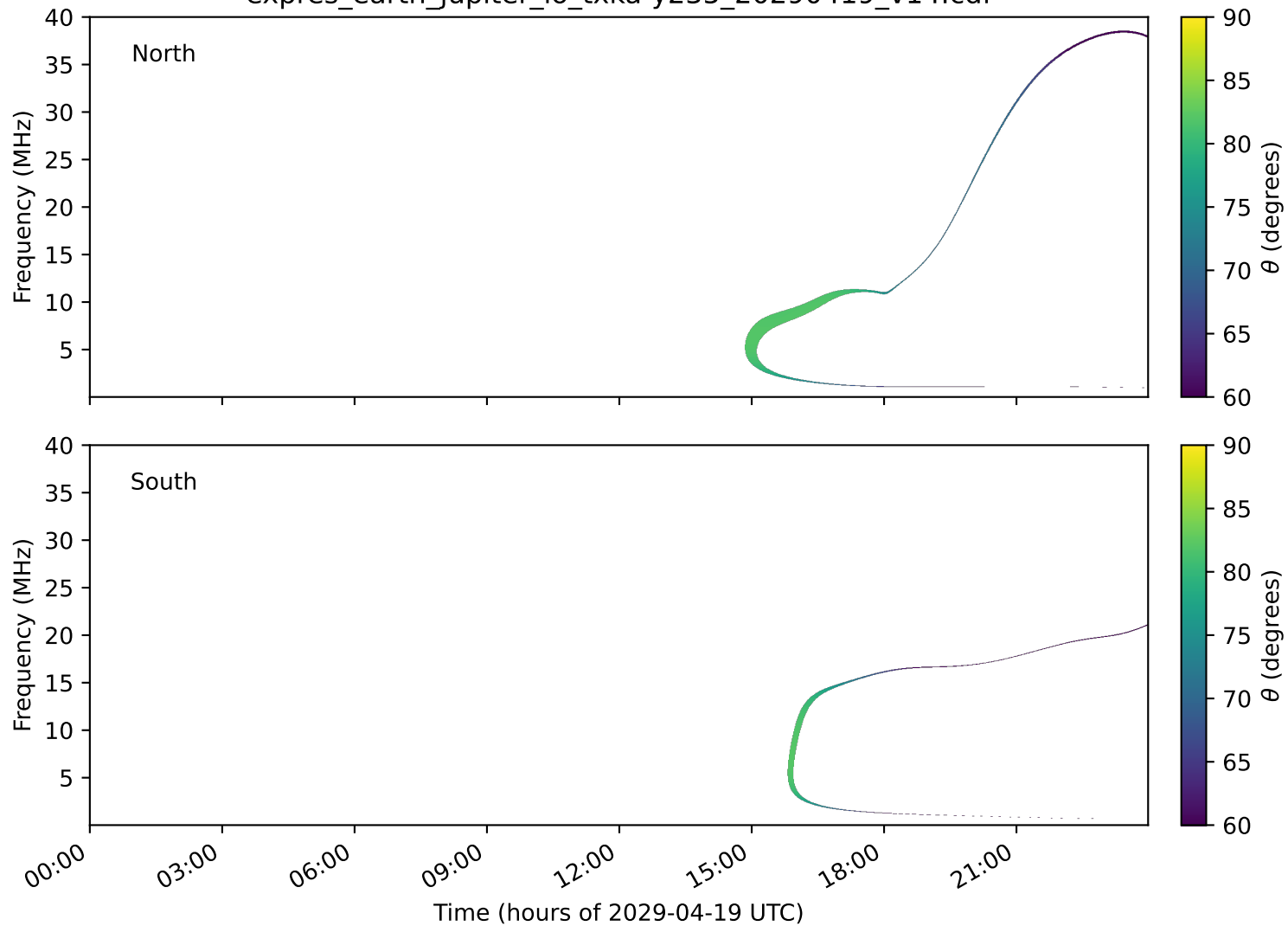
expres_earth_jupiter_io_txka-y235_20290419_v14.cdf
