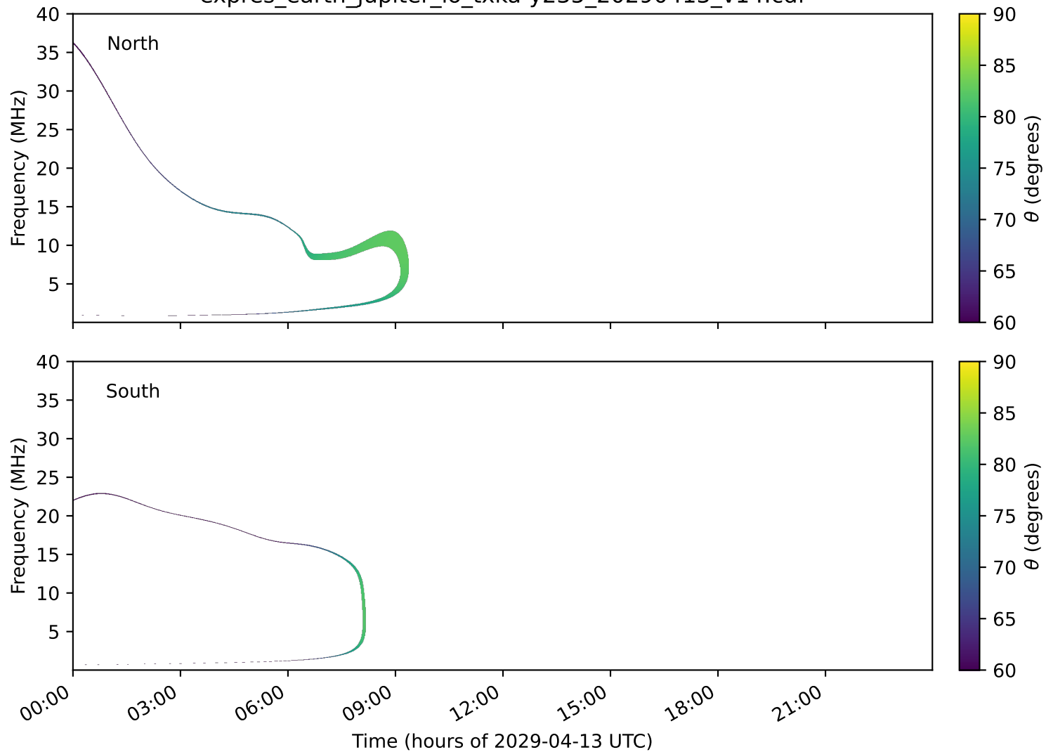
expres_earth_jupiter_io_txka-y235_20290413_v14.cdf
