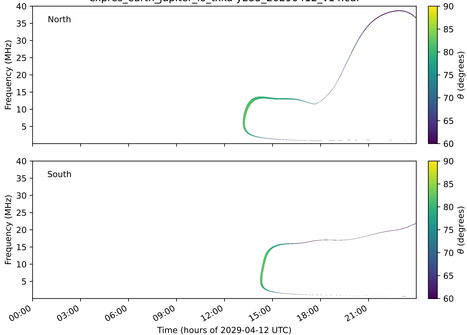
expres_earth_jupiter_io_txka-y235_20290412_v14.cdf
