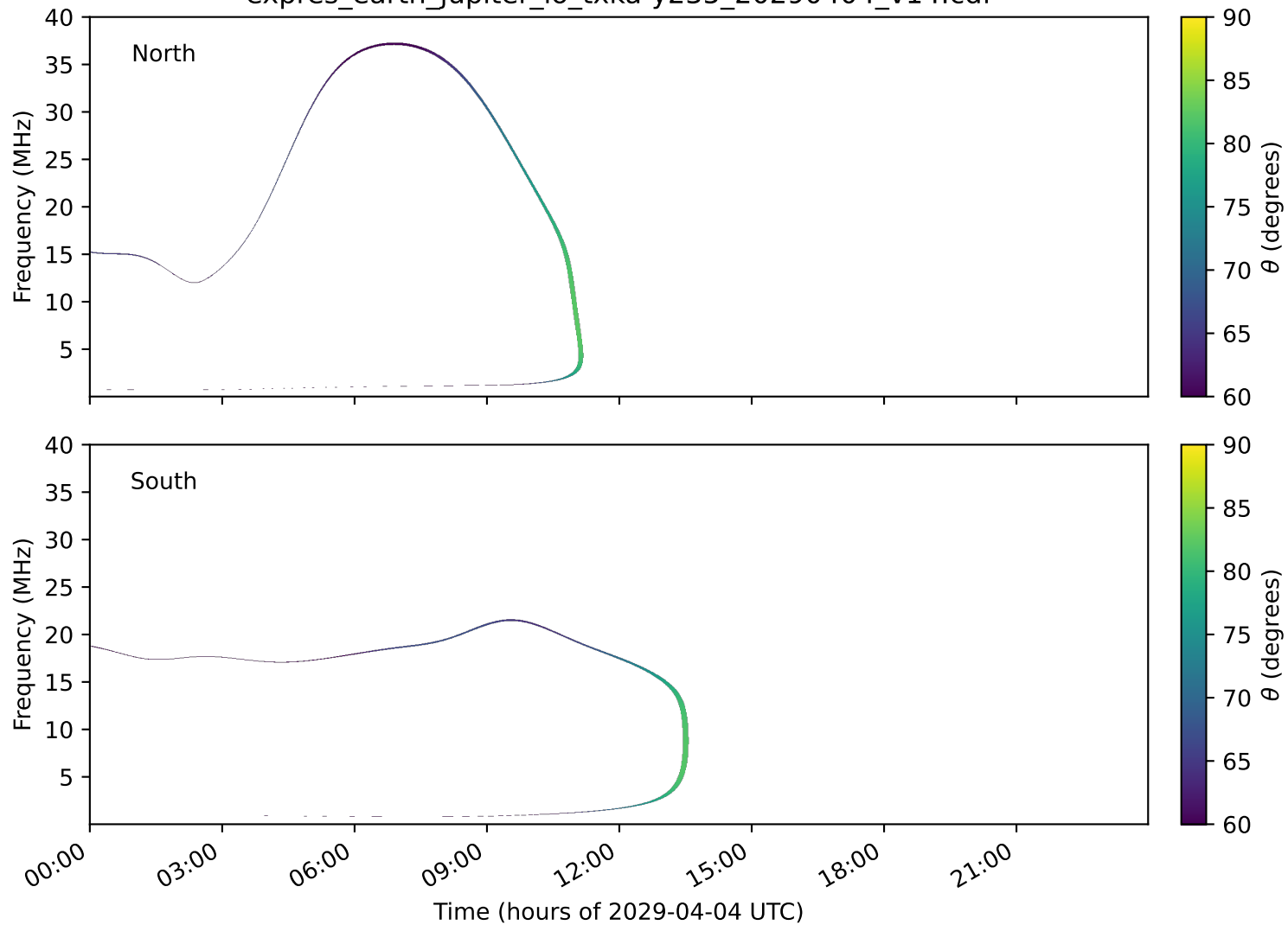
expres_earth_jupiter_io_txka-y235_20290404_v14.cdf
