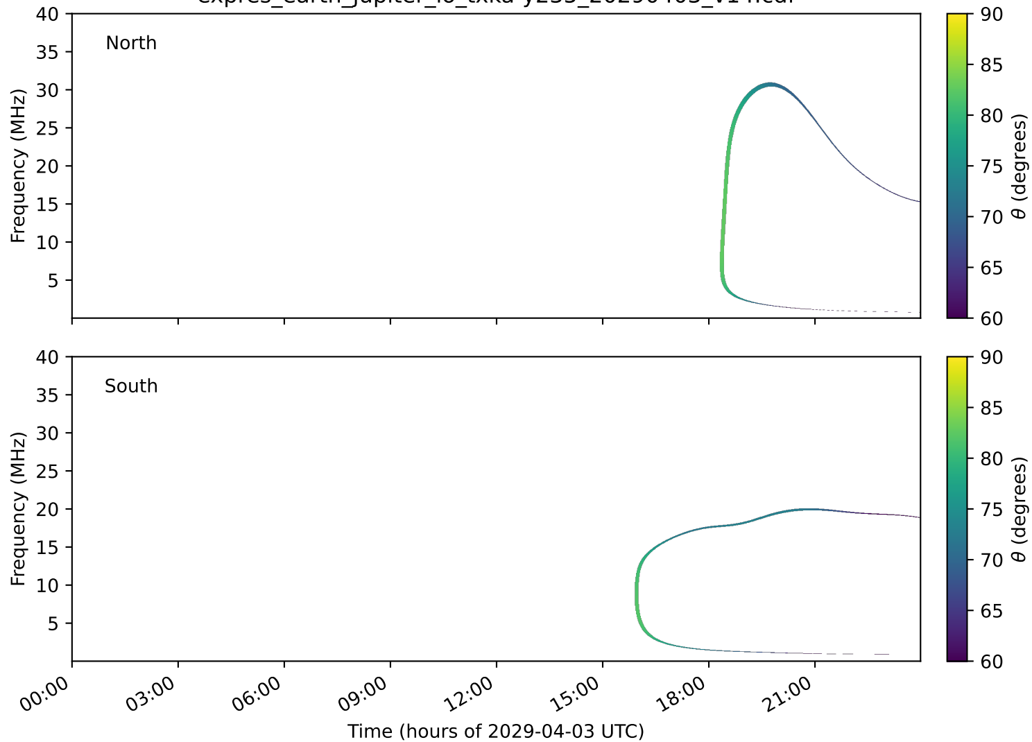
expres_earth_jupiter_io_txka-y235_20290403_v14.cdf
