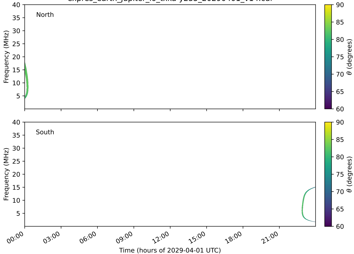
expres_earth_jupiter_io_txka-y235_20290401_v14.cdf
