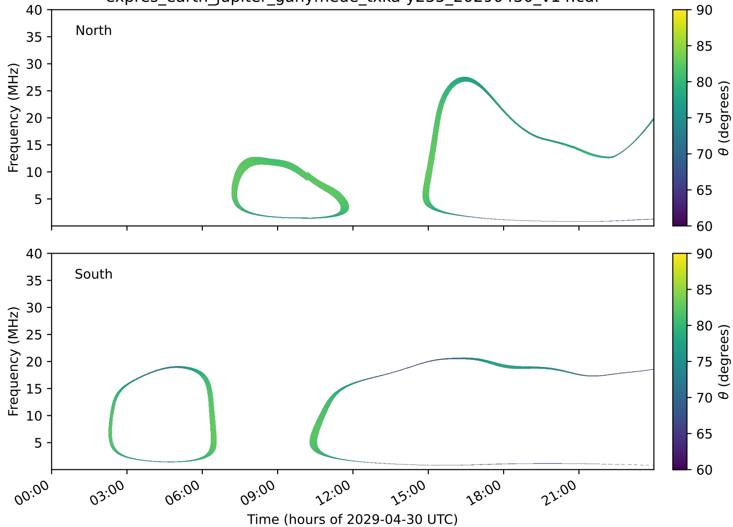
expres_earth_jupiter_ganymede_txka-y235_20290430_v14.cdf
