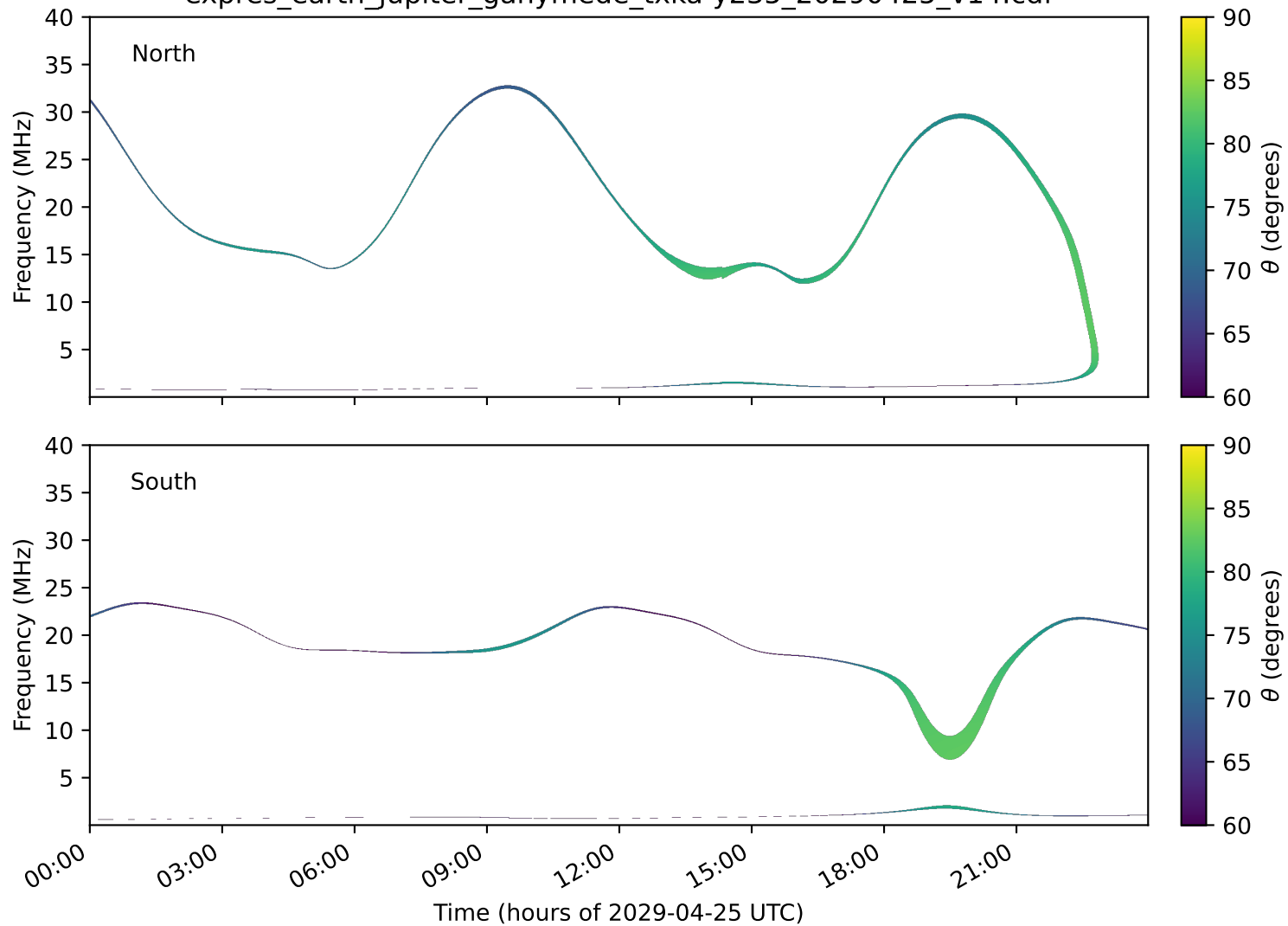
expres_earth_jupiter_ganymede_txka-y235_20290425_v14.cdf
