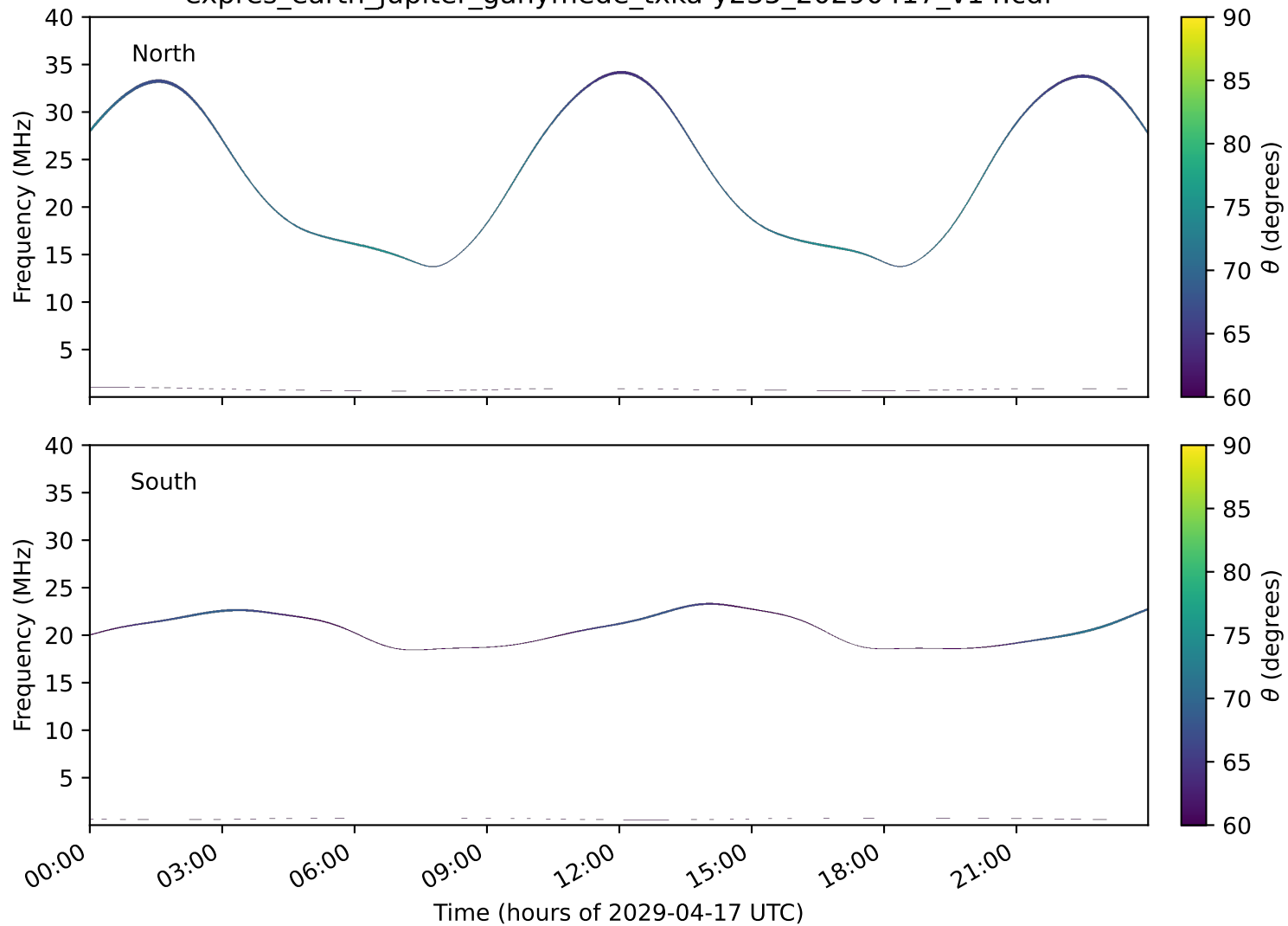
expres_earth_jupiter_ganymede_txka-y235_20290417_v14.cdf
