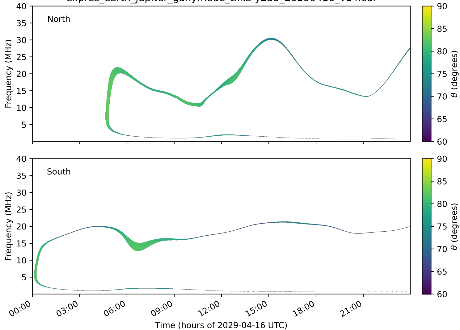
expres_earth_jupiter_ganymede_txka-y235_20290416_v14.cdf
