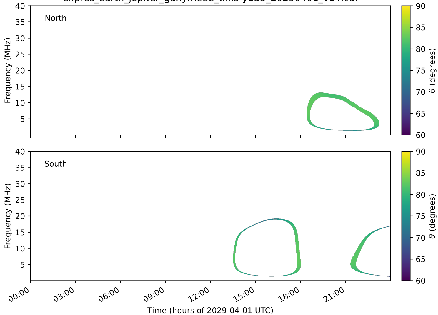
expres_earth_jupiter_ganymede_txka-y235_20290401_v14.cdf
