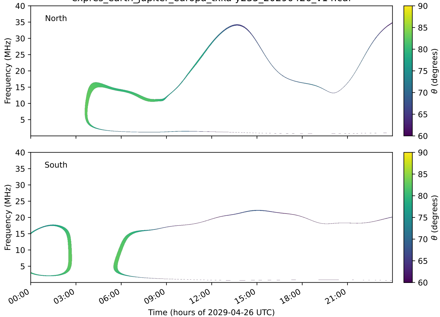
expres_earth_jupiter_europa_txka-y235_20290426_v14.cdf
