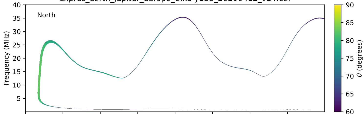
expres_earth_jupiter_europa_txka-y235_20290412_v14.cdf
