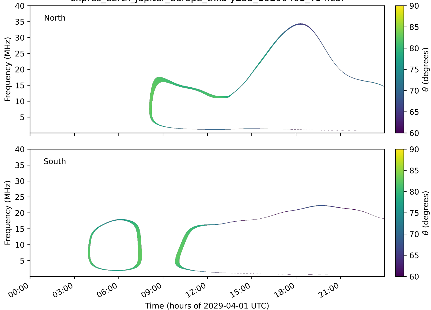
expres_earth_jupiter_europa_txka-y235_20290401_v14.cdf
