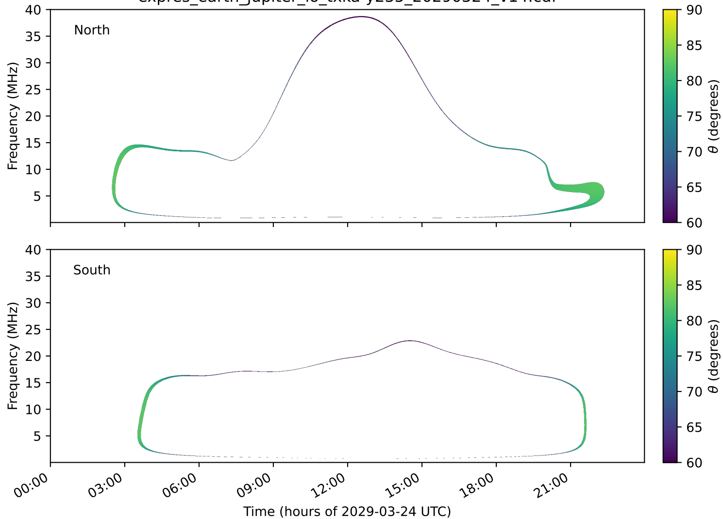
expres_earth_jupiter_io_txka-y235_20290324_v14.cdf
