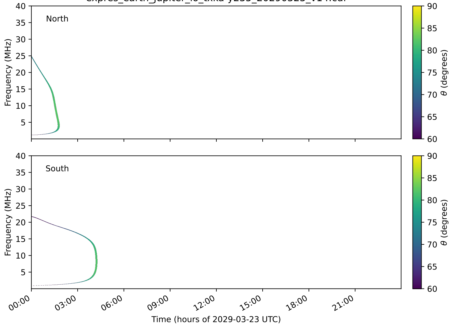
expres_earth_jupiter_io_txka-y235_20290323_v14.cdf
