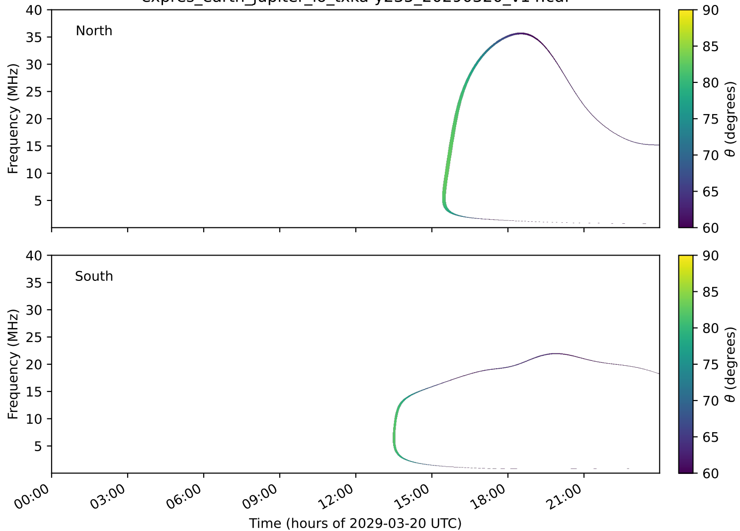
expres_earth_jupiter_io_txka-y235_20290320_v14.cdf
